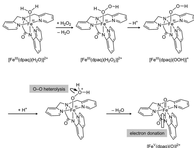
Scheme 2. Formation of the Fe V oxo species from complex 1 .
