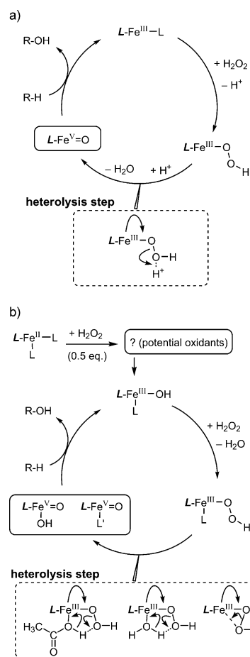
Scheme 3. Catalytic cycles of hydroxylation with a) Fe III –dpaq, and b) an Fe II complex with two cis -oriented labile sites.
